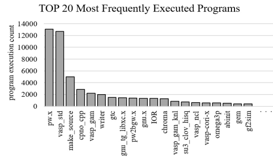
Figure 3: Top 20 mostly executed programs
