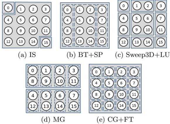
Figure 4: Topology of Different Benchmarks for 16 Processes Through Call-path+Parameter Clustering
