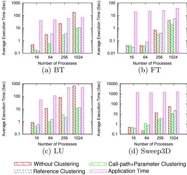
Figure 8: Execution Overhead - Nodes/Tasks=1/16
