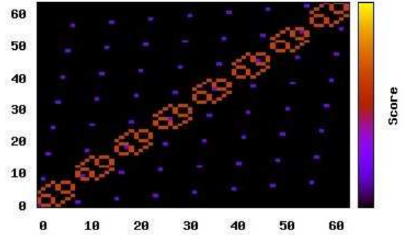
Figure 6: CG Communication Matrix
