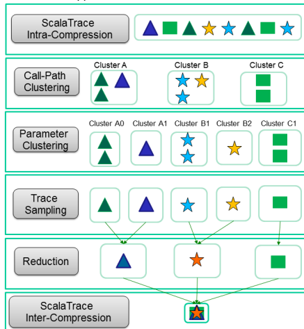
Figure 3: Overview of Proposed Clustering Algorithm
