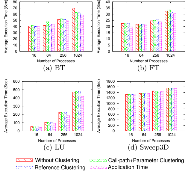
Figure 9: Replay Time of Traces - Weak Scaling - Nodes/Tasks=1/16
