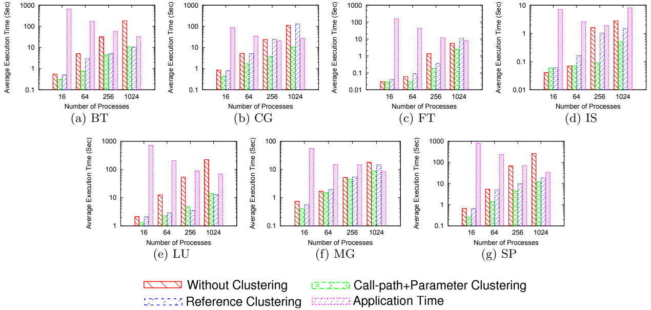
Figure 5: Execution Overhead for NAS benchmarks - Strong Scaling - Nodes/Tasks=1/16
