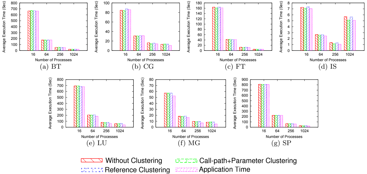
Figure 7: Replay Time of Traces - Strong Scaling - Nodes/Tasks=1/16
