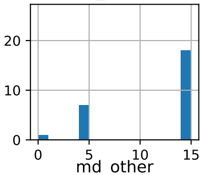
file_create
