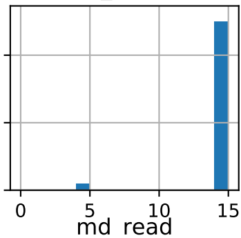
file_delete
