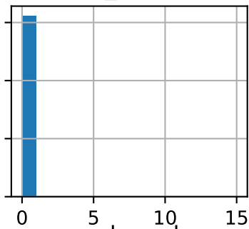
md_read
