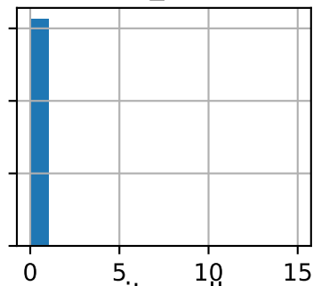
write_calls
