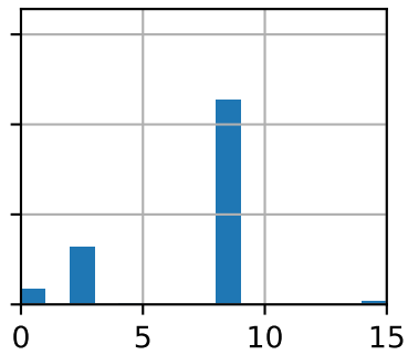
write_calls
