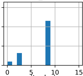
write_bytes
